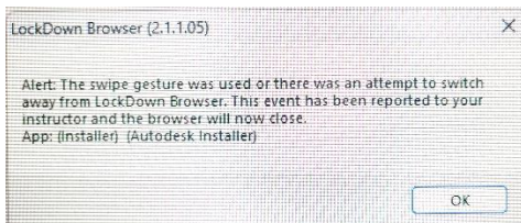
Fig 14: Alert
