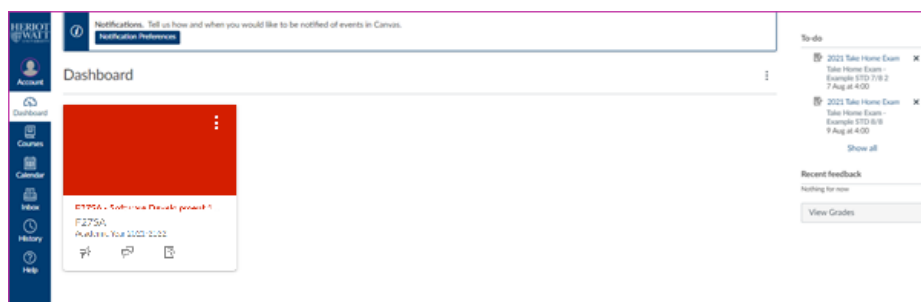
Fig 2: Dashboard
