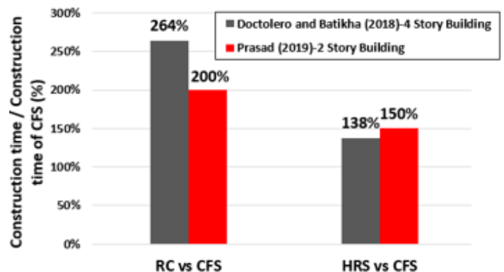
Fig. 7. CFS vs RC and HRS in terms of the Construction Duration
