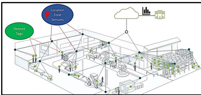
Fig. 4. RFID Network.
