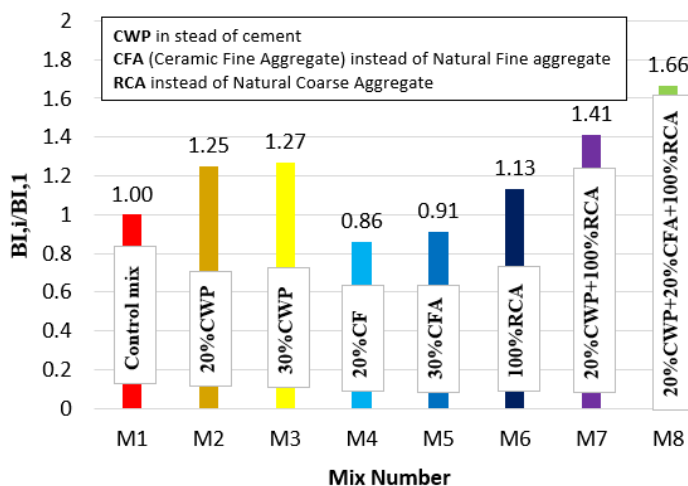
Fig. 5. The relative differences in the Beneficial index for each mix in comparison with (M1).
