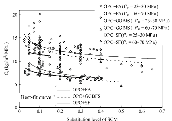
Fig. 1. Effect of substitution level of SCM on CO 2 intensity ( C_i ) [8].
