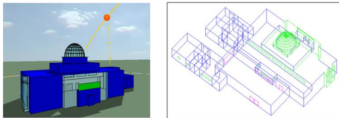
Fig.3. IESVE model of Abdul Rahman Siddique Mosque. Left image: 3D model with sun path and shadows. Right image: Axonometric view of the model geometry
