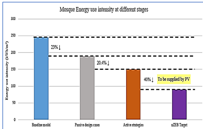
Fig. 2. IES mosque's EUI at different stages of retrofit solutions. Reductions in energy consumption due to each stage is also shown in percentages.
