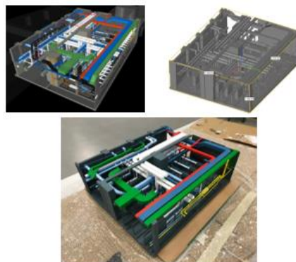
Fig. 1. BIM model vs digital 3D printing model and the final 3D printed product.
