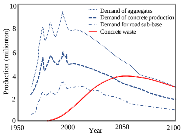
Fig. 2. Estimation of concrete waste and aggregate demand in Japan [11].
