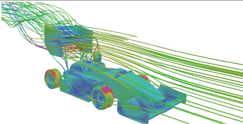
Simulation of Air Stream over a Formula Student Car [SimScale]
