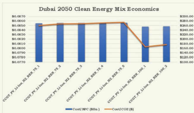
Fig. 7 Economic indicators for 2050 scenario.
