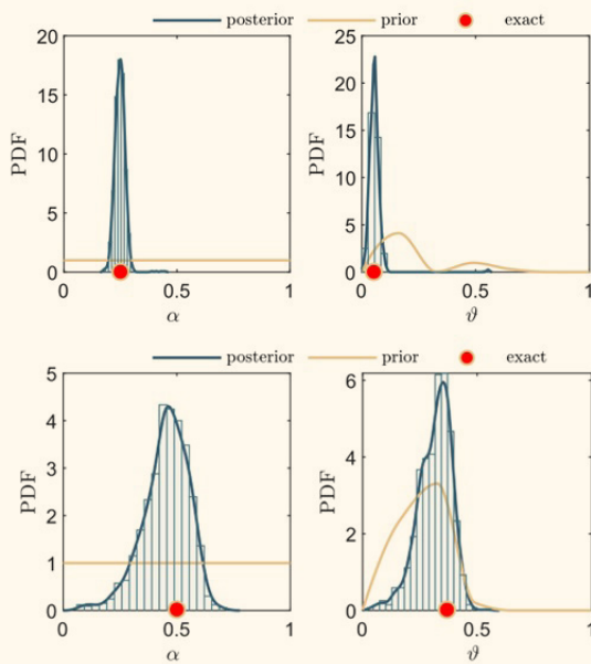
Fig. 4 Identified damage severity \alpha , and damage location \theta , using the FDI algorithm for the noise of 1% (top), and 5% (bottom) [29].
